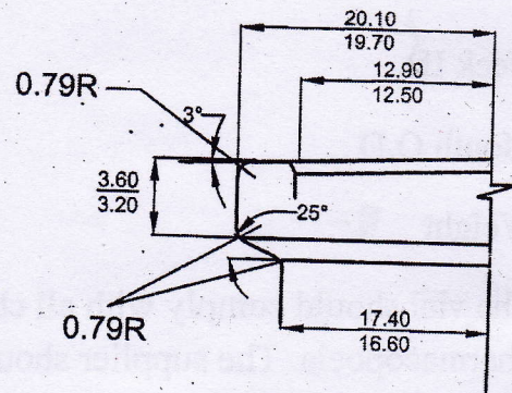
NECK FINISH DETAIL
